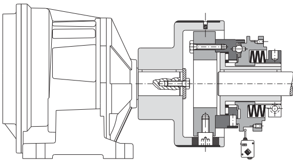
Model DSS or DSR with compact elastic coupling GEC for coaxial shaft transmission.
