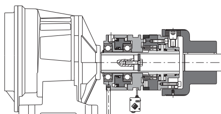
Model DSR/F/AP with Compact elastic coupling GEC for coaxial shaft transmission.
