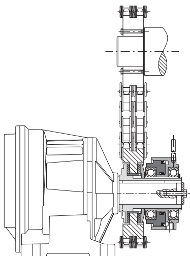
Model DSF/TF/AP with plate wheel for parallel shaft transmission.
