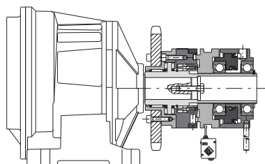
Model DSR/TF/AP with plate wheel for parallel shaft transmission.
